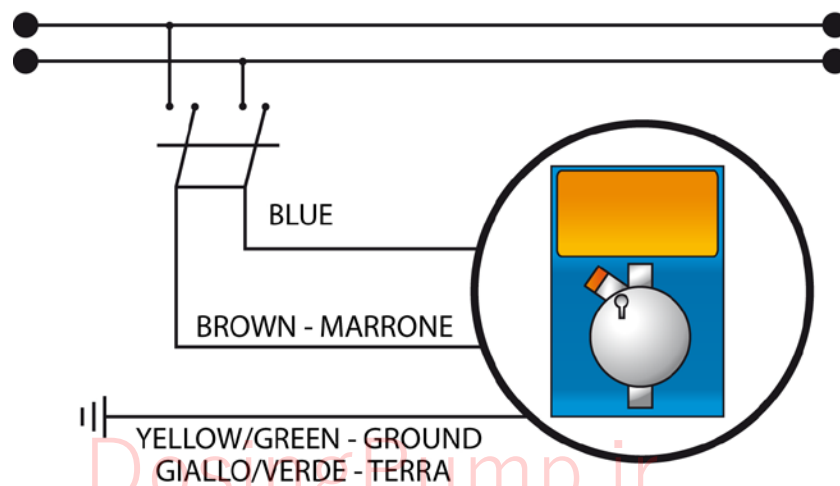
Fig.3 – Electrical Connection
